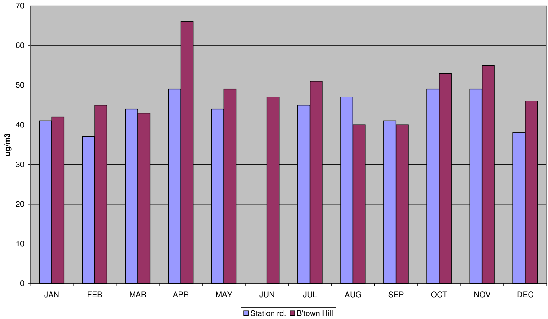
Nitrogen Dioxide diffusion tube results, Totnes locations, 2007.
