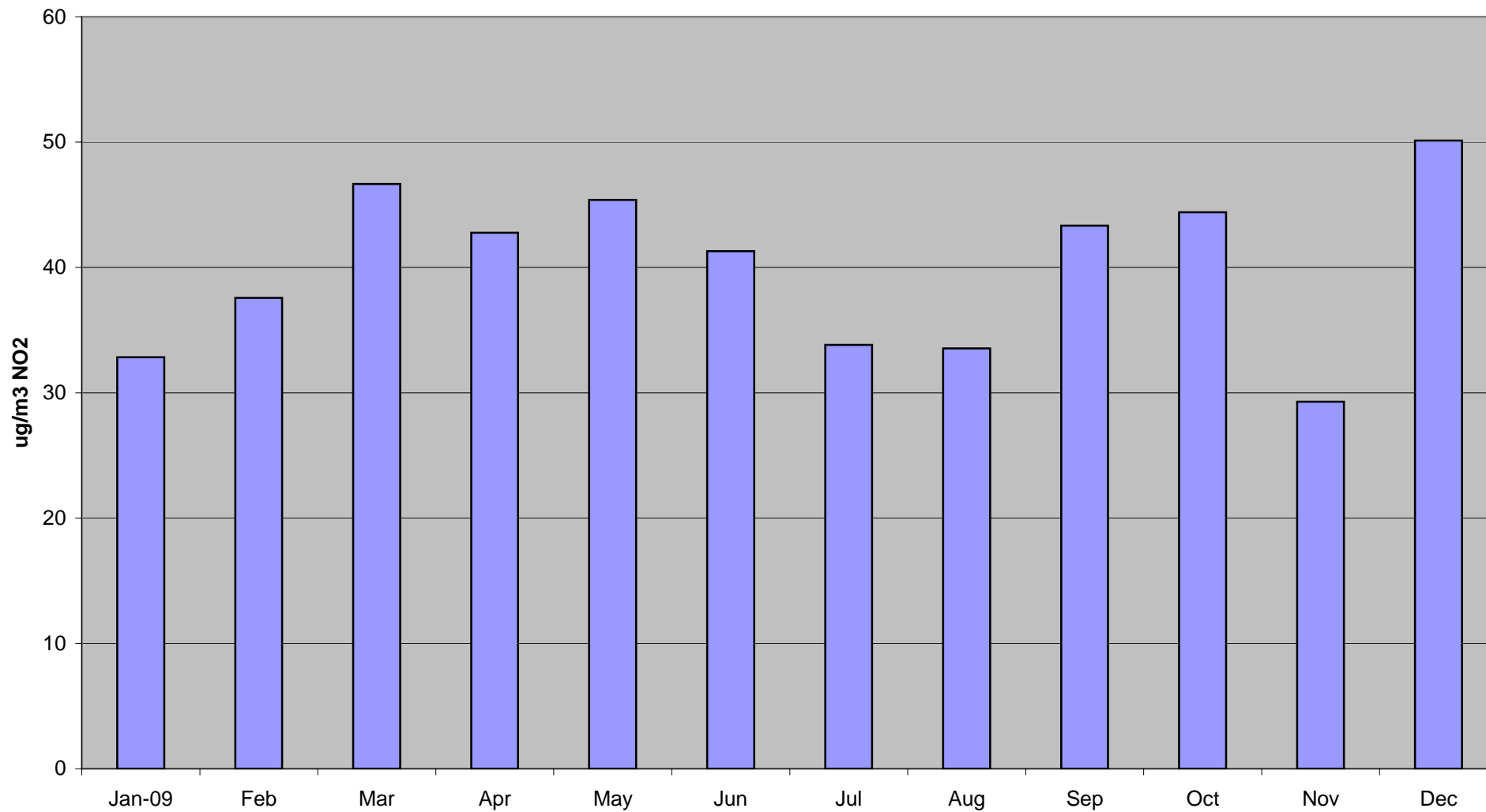
NO2 Levels; Kingsbridge Fore Street, 2009
