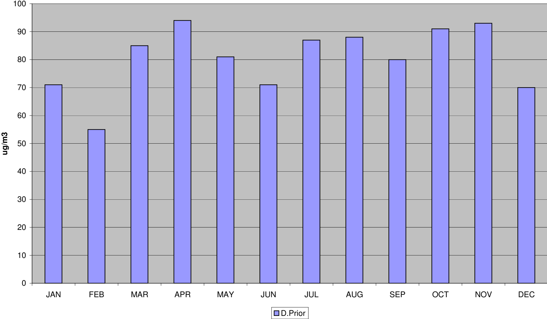
Nitrogen Dioxide diffusion tube results - A38 at Dean Prior, 2007
